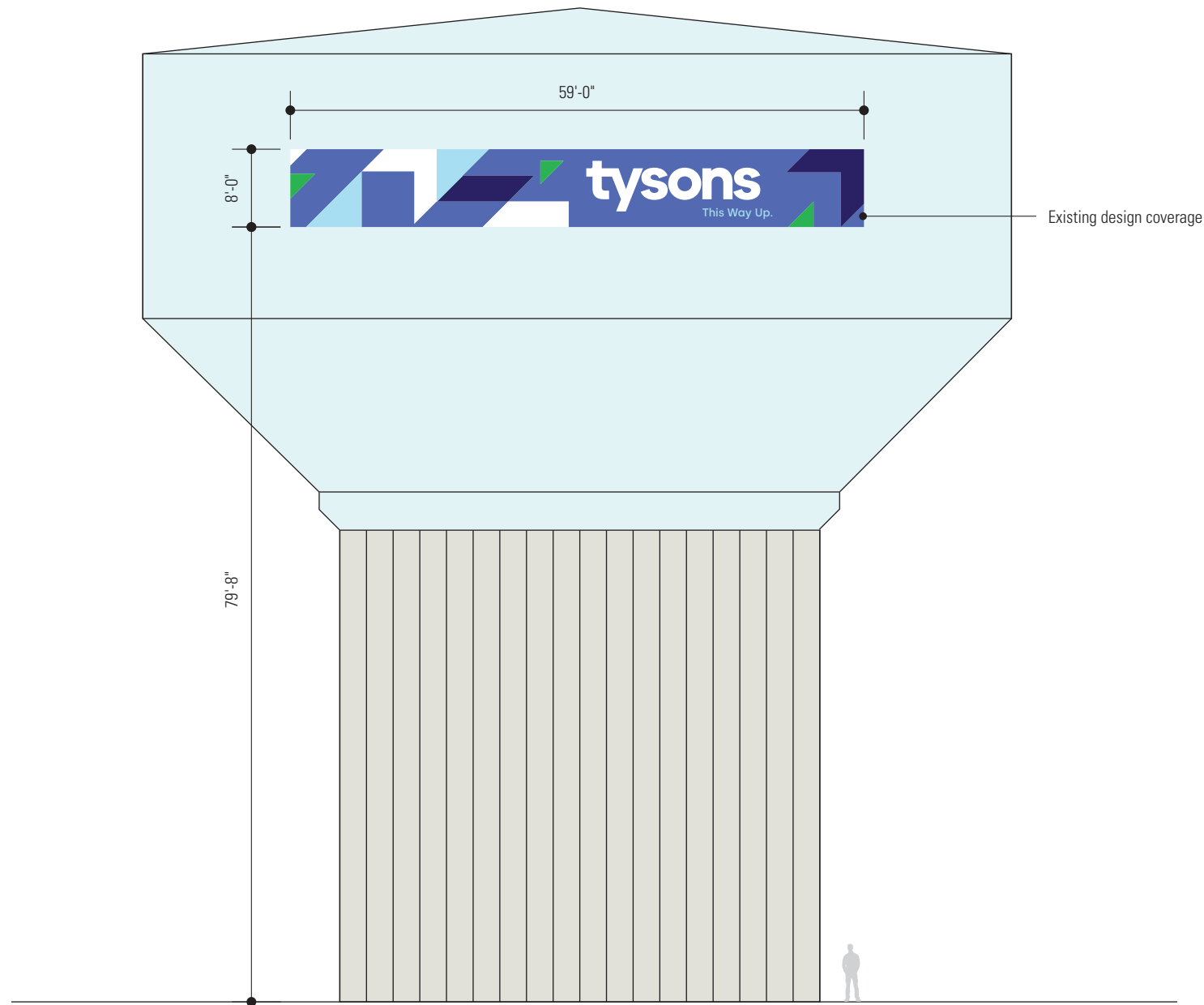
A ELEVATION: SOUTHWEST SCALE: 3/4"=1'-0"
